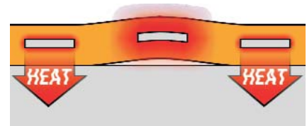
Voids or bubbles beneath the heater cause localized hot spots which can result in premature heater failure
