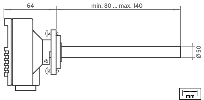
GMD20 Dimensions
