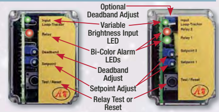
API 1600 G AC Input Alarms
